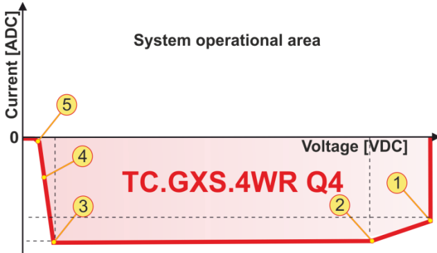
Q4 range of device TC.GXS.20.400.4WR.S.
