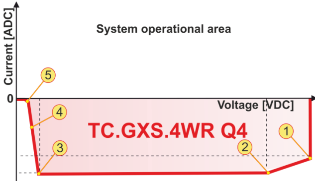
Q4 range of device TC.GXS.32.400.4WR.S.
