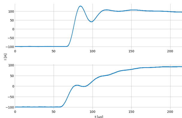
Figure 2: Parameterization example: set-value step currents. -97...97 A@333VDC in <50 \mu s with overshoot (top), in <200 \mu s w/o overshoot (bottom).
